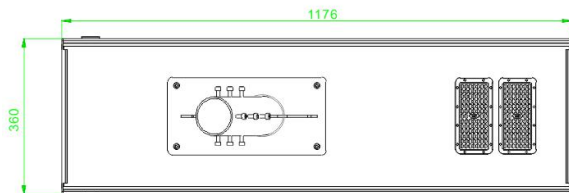
6040P(Size:1176*360*60)
