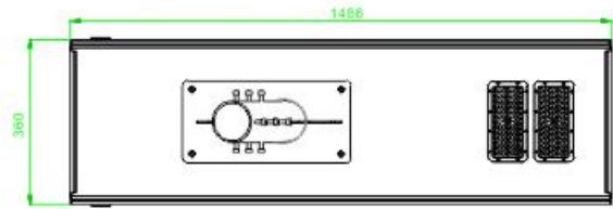
8060P(Size:1486*360*60)
